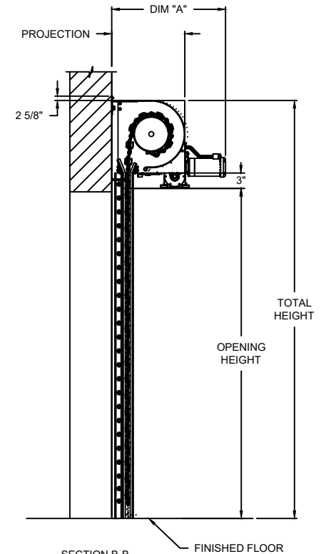
SECTION B-B
