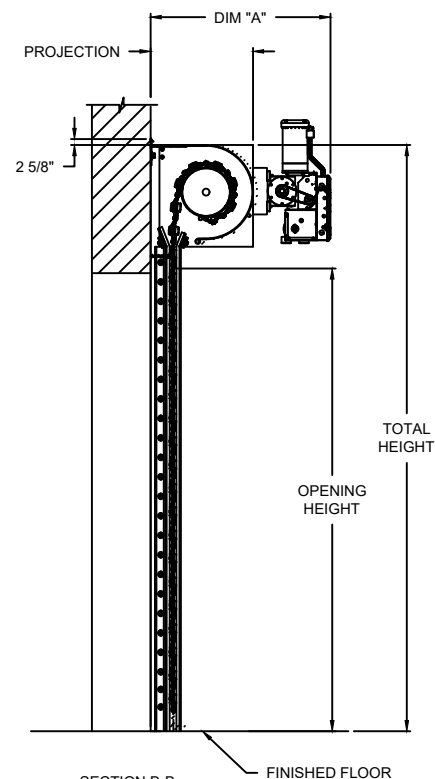
SECTION B-B
