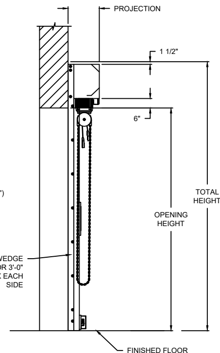
SECTION B-B
